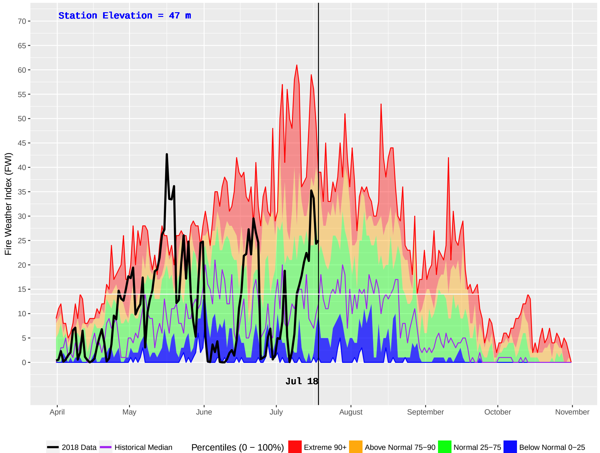
HAGENSBORG 2 (904) : Historical (2005–2016) and Current (2018) Daily Fire Weather Index (FWI)
