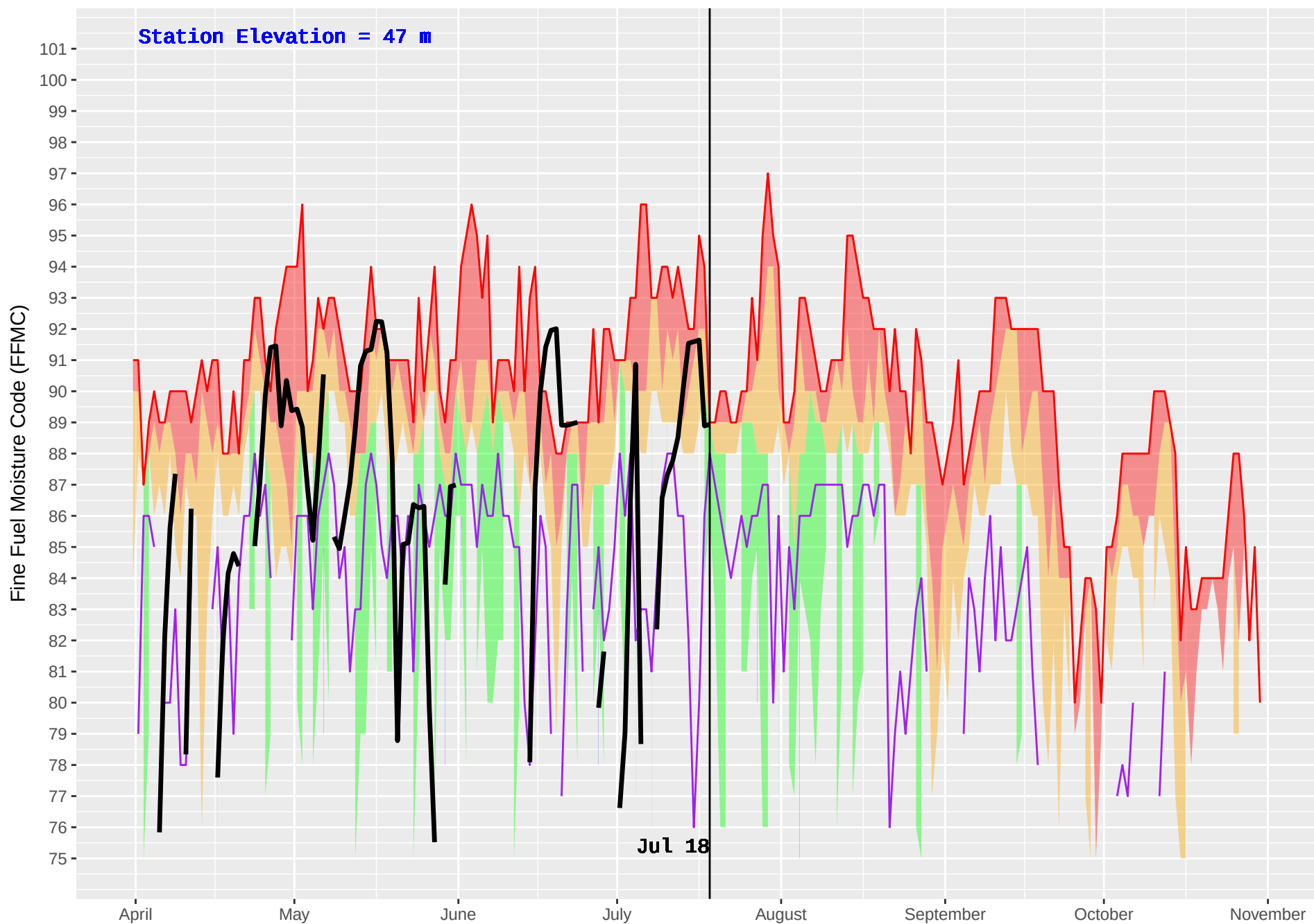
HAGENSBORG 2 (904) : Historical (2005–2016) and Current (2018) Daily Fine Fuel Moisture Code (FFMC)
